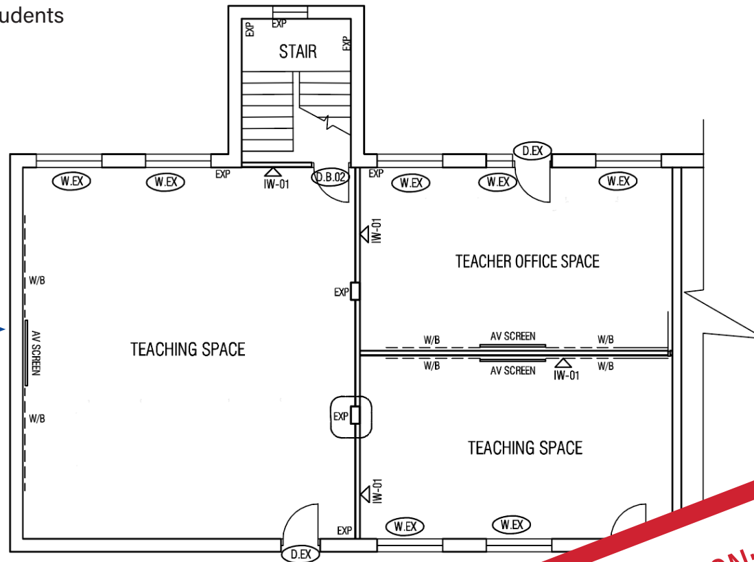
GROUND FLOOR PLAN BORONIA
